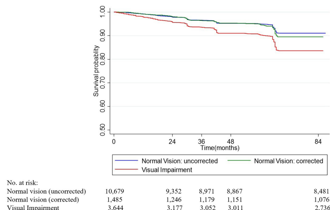
Figure 3 Kaplan-Meier survival curves (2011–2018).
